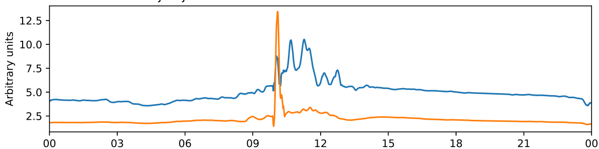
Tjautjas 30 MHz and 38 MHz riometer 2025-11-11 UTC
