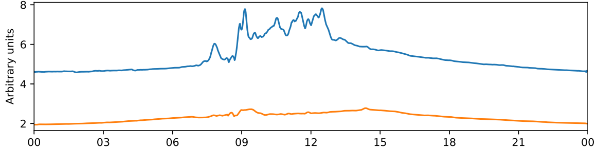
Tjautjas 30 MHz and 38 MHz riometer 2025-11-15 UTC
