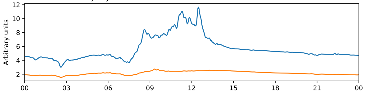
Tjautjas 30 MHz and 38 MHz riometer 2025-11-17 UTC
