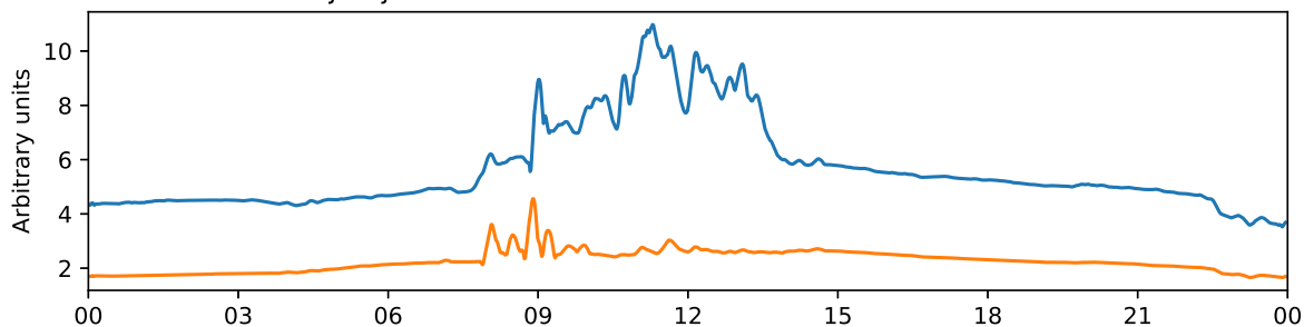
Tjautjas 30 MHz and 38 MHz riometer 2025-11-10 UTC
