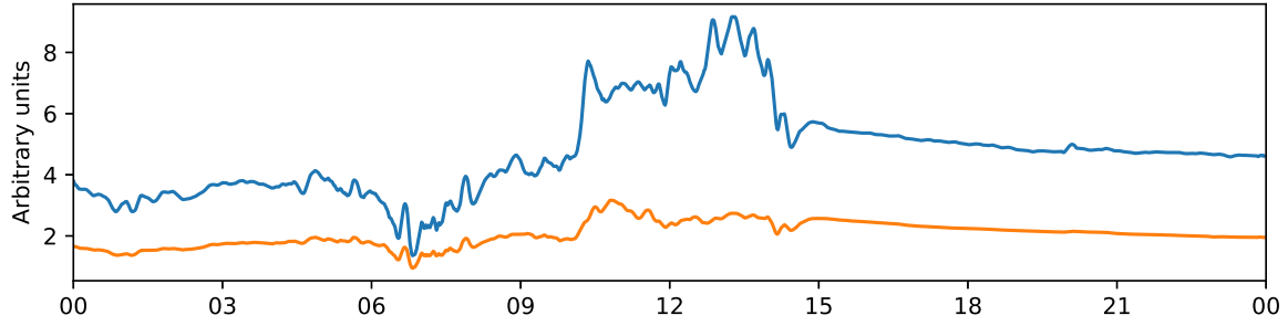
Tjautjas 30 MHz and 38 MHz riometer 2025-11-14 UTC
