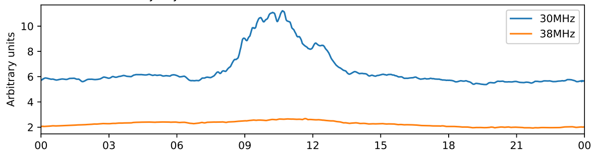
Tjautjas 30 MHz and 38 MHz riometer 2025-12-31 UTC
