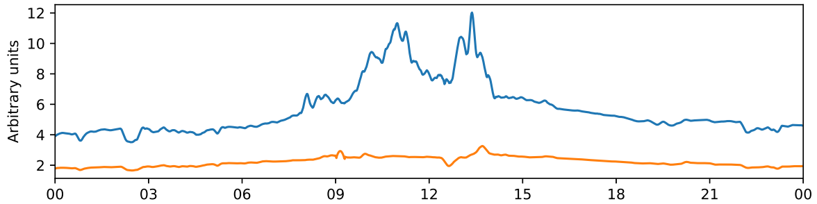
Tjautjas 30 MHz and 38 MHz riometer 2025-11-17 UTC
