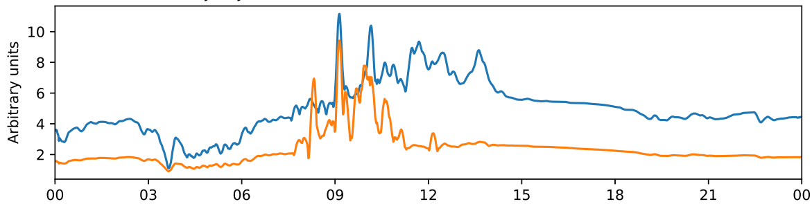
Tjautjas 30 MHz and 38 MHz riometer 2025-11-08 UTC
