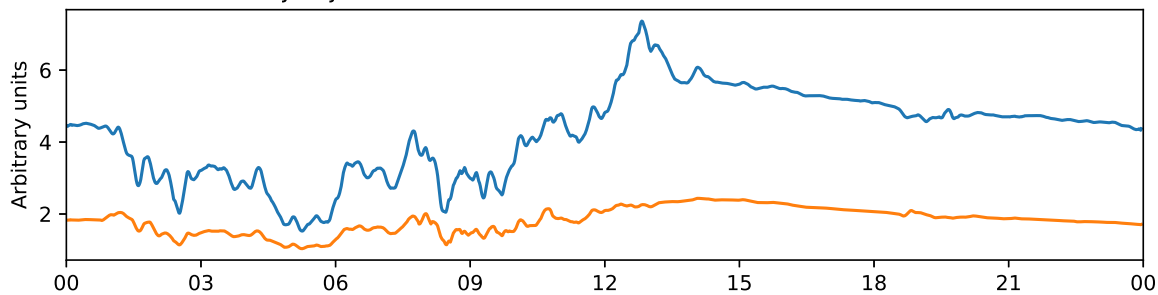
Tjautjas 30 MHz and 38 MHz riometer 2025-11-09 UTC
