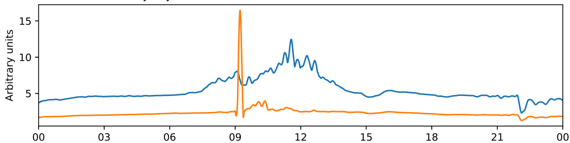
Tjautjas 30 MHz and 38 MHz riometer 2025-11-11 UTC
