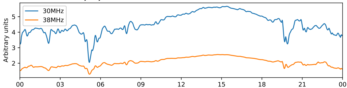
Tjautjas 30 MHz and 38 MHz riometer 2025-11-07 UTC
