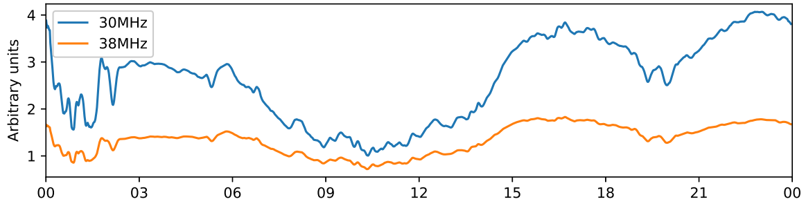
Tjautjas 30 MHz and 38 MHz riometer 2025-11-13 UTC
