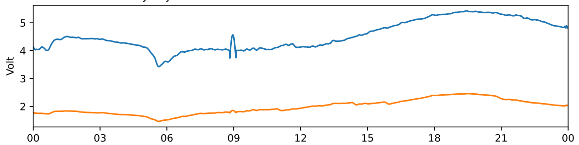
Tjautjas 30 MHz and 38 MHz riometer 2025-08-23 UTC
