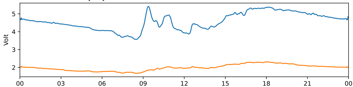
Tjautjas 30 MHz and 38 MHz riometer 2025-09-13 UTC
