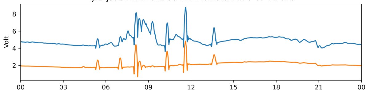
Tjautjas 30 MHz and 38 MHz riometer 2025-09-04 UTC
