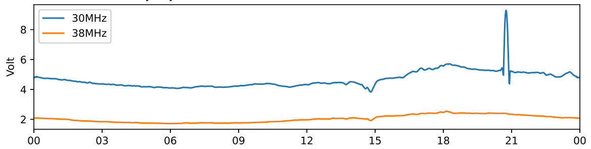
Tjautjas 30 MHz and 38 MHz riometer 2025-08-19 UTC
