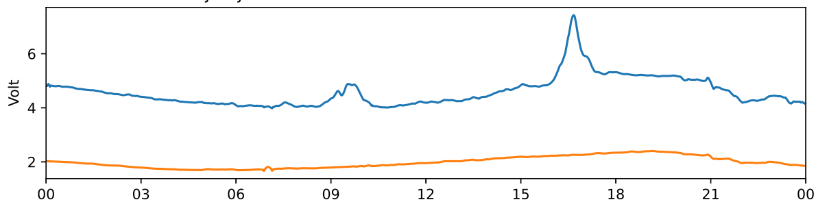
Tjautjas 30 MHz and 38 MHz riometer 2025-09-02 UTC
