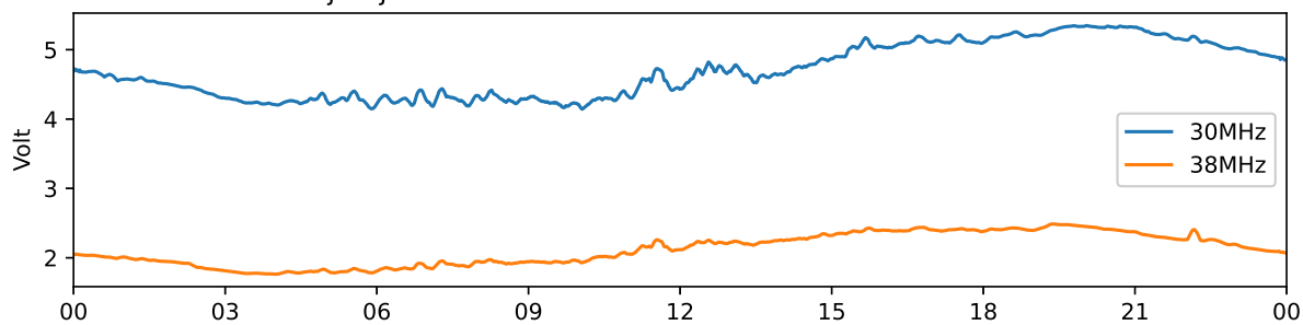
Tjautjas 30 MHz and 38 MHz riometer 2025-08-31 UTC
