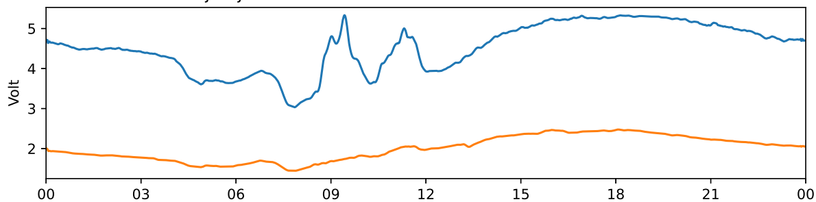
Tjautjas 30 MHz and 38 MHz riometer 2025-09-14 UTC
