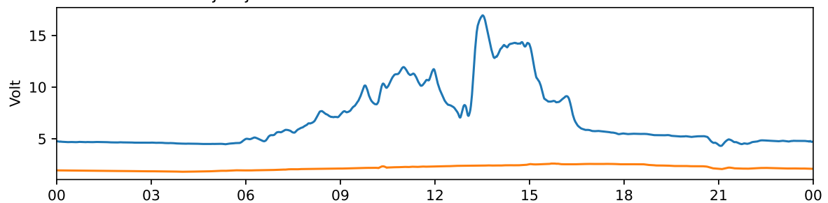
Tjautjas 30 MHz and 38 MHz riometer 2025-09-22 UTC
