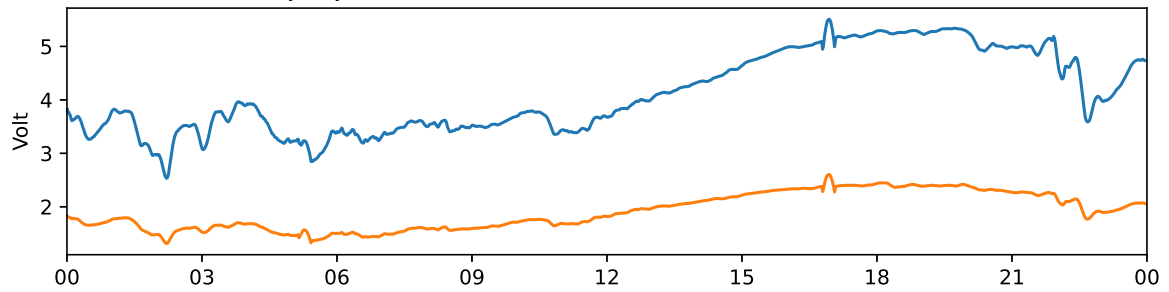
Tjautjas 30 MHz and 38 MHz riometer 2025-08-21 UTC
