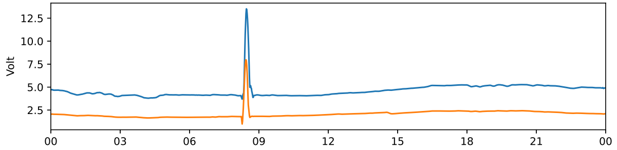
Tjautjas 30 MHz and 38 MHz riometer 2025-08-22 UTC
