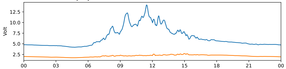
Tjautjas 30 MHz and 38 MHz riometer 2025-09-22 UTC
