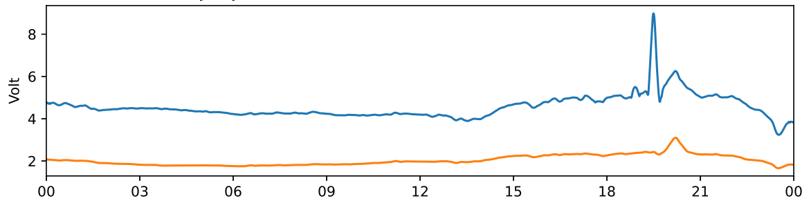
Tjautjas 30 MHz and 38 MHz riometer 2025-08-20 UTC
