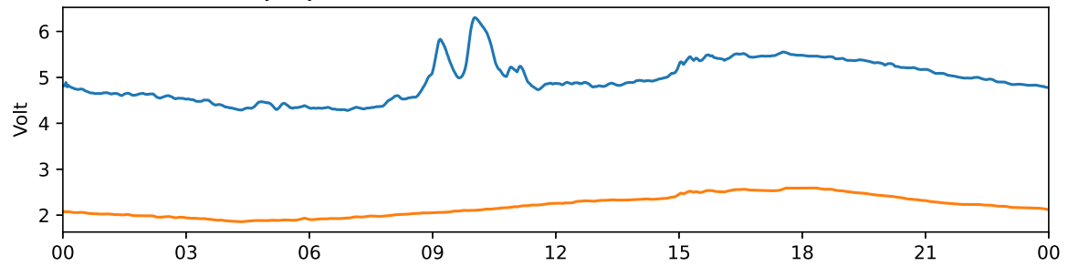
Tjautjas 30 MHz and 38 MHz riometer 2025-09-20 UTC
