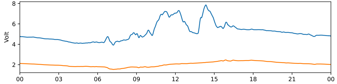
Tjautjas 30 MHz and 38 MHz riometer 2025-09-21 UTC
