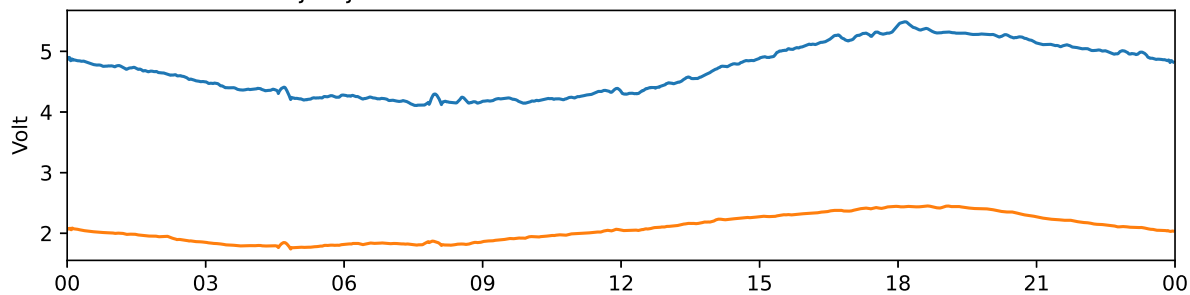
Tjautjas 30 MHz and 38 MHz riometer 2025-09-01 UTC
