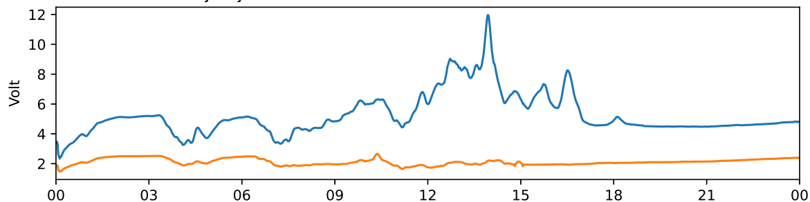
Tjautjas 30 MHz and 38 MHz riometer 2025-03-16 UTC
