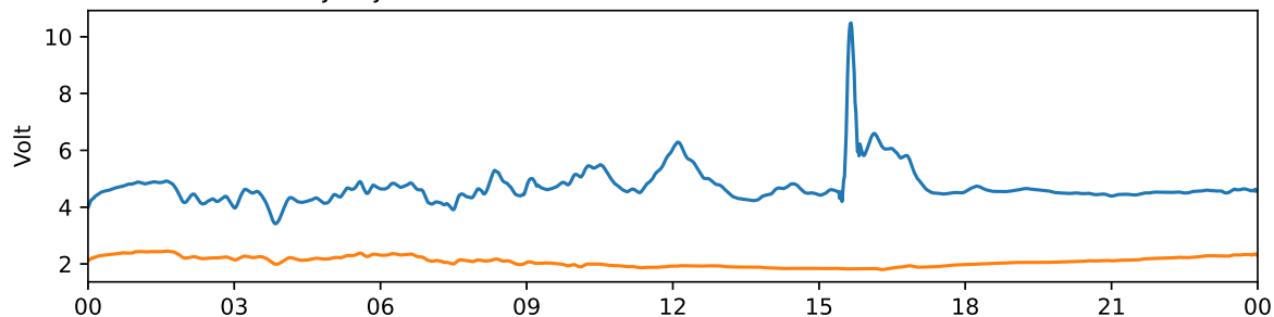
Tjautjas 30 MHz and 38 MHz riometer 2025-03-19 UTC
