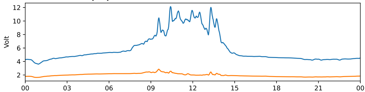
Tjautjas 30 MHz and 38 MHz riometer 2025-01-30 UTC
