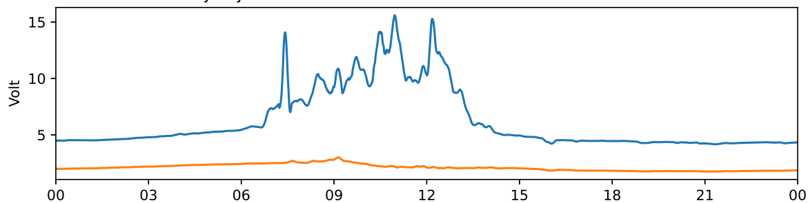
Tjautjas 30 MHz and 38 MHz riometer 2025-01-28 UTC
