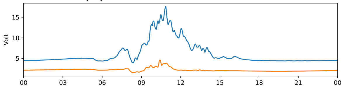
Tjautjas 30 MHz and 38 MHz riometer 2025-02-09 UTC
