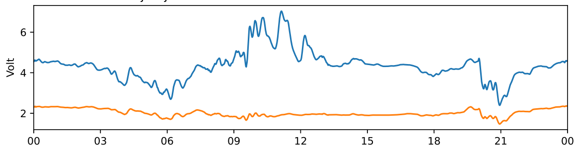
Tjautjas 30 MHz and 38 MHz riometer 2025-03-19 UTC
