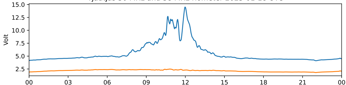
Tjautjas 30 MHz and 38 MHz riometer 2025-01-18 UTC
