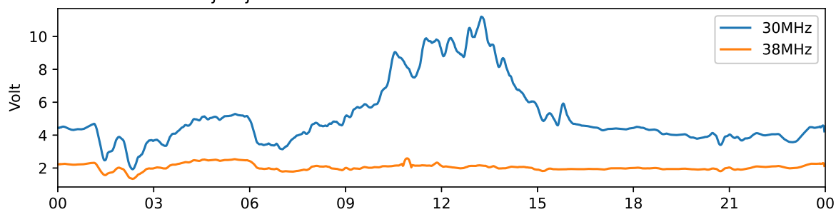
Tjautjas 30 MHz and 38 MHz riometer 2025-03-15 UTC
