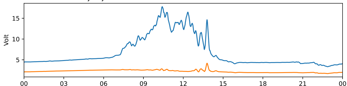
Tjautjas 30 MHz and 38 MHz riometer 2025-02-10 UTC
