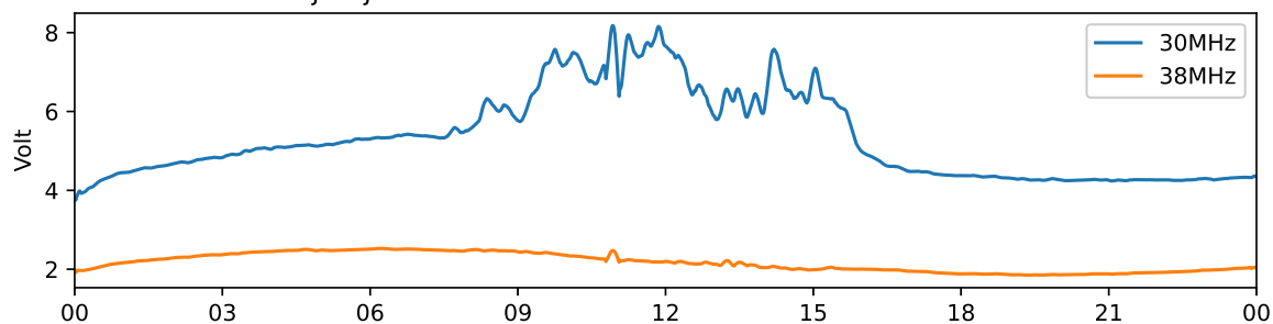
Tjautjas 30 MHz and 38 MHz riometer 2025-02-07 UTC
