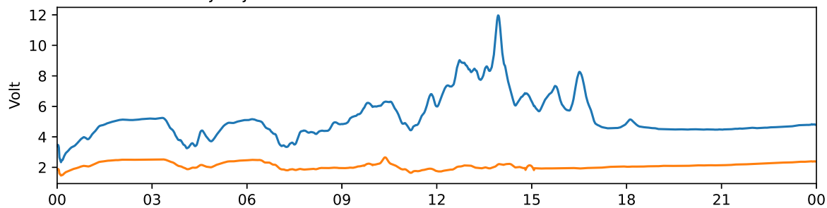
Tjautjas 30 MHz and 38 MHz riometer 2025-03-16 UTC
