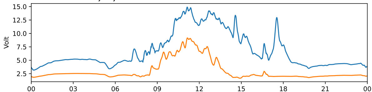
Tjautjas 30 MHz and 38 MHz riometer 2025-03-18 UTC
