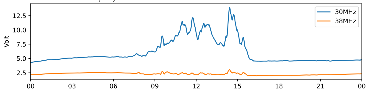
Tjautjas 30 MHz and 38 MHz riometer 2025-03-03 UTC
