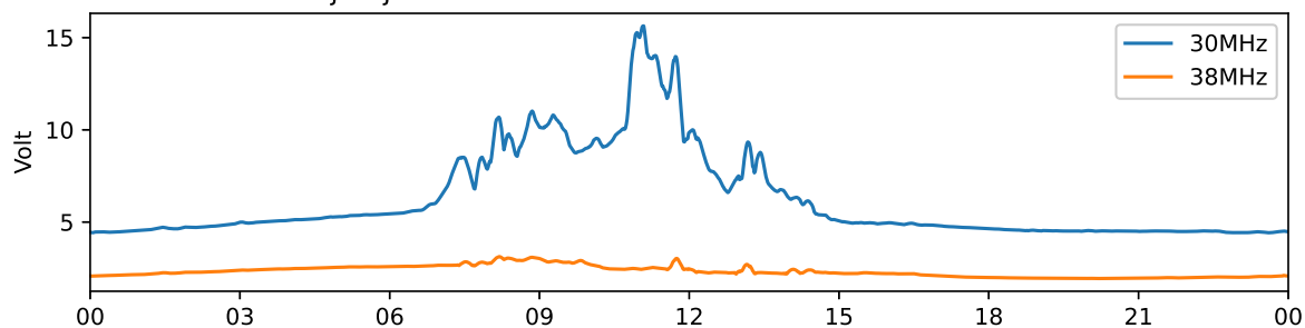
Tjautjas 30 MHz and 38 MHz riometer 2025-01-26 UTC
