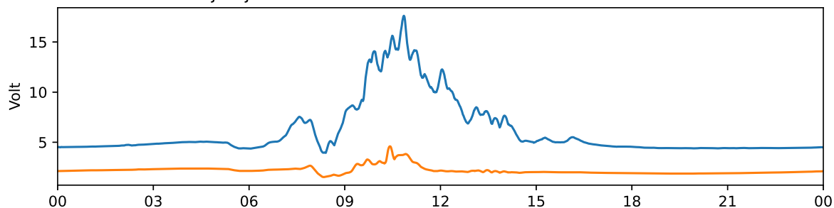
Tjautjas 30 MHz and 38 MHz riometer 2025-02-09 UTC
