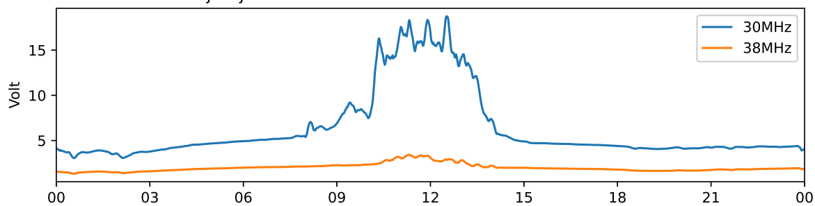
Tjautjas 30 MHz and 38 MHz riometer 2025-01-14 UTC
