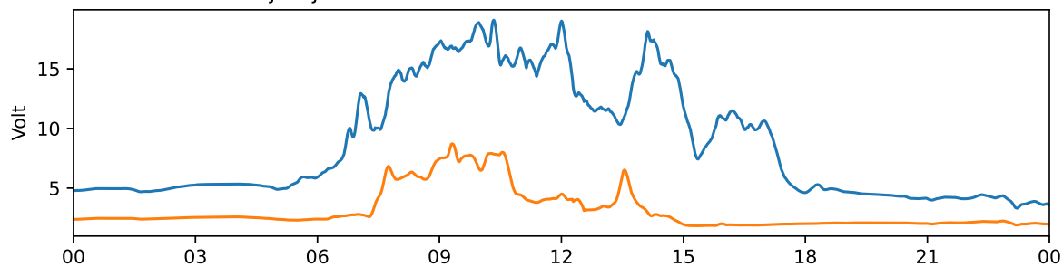
Tjautjas 30 MHz and 38 MHz riometer 2025-03-17 UTC
