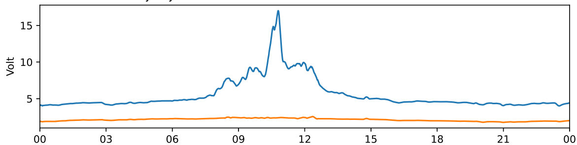
Tjautjas 30 MHz and 38 MHz riometer 2025-01-15 UTC
