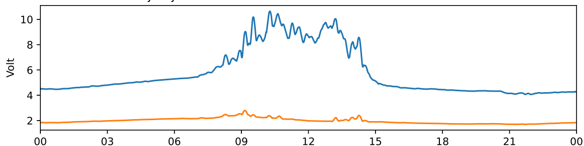
Tjautjas 30 MHz and 38 MHz riometer 2025-01-30 UTC
