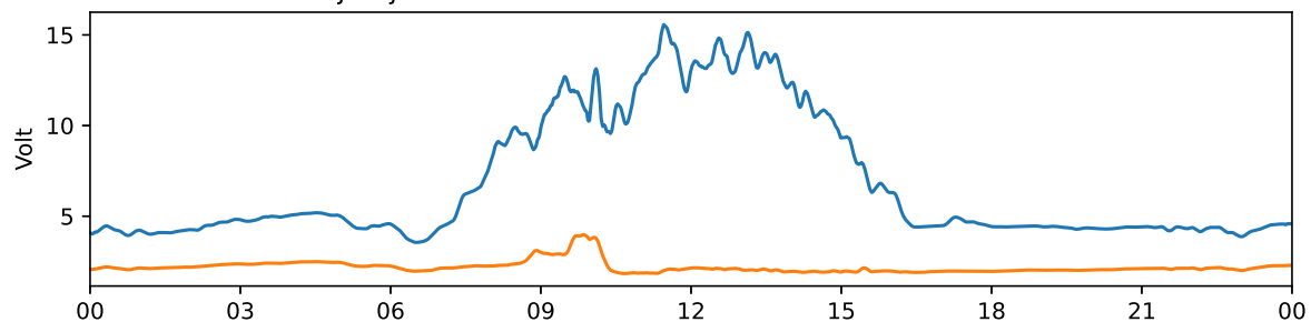
Tjautjas 30 MHz and 38 MHz riometer 2025-03-06 UTC
