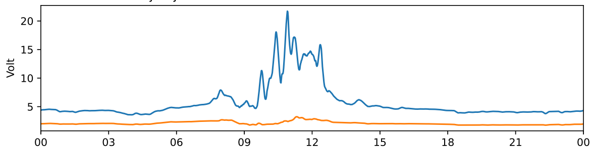
Tjautjas 30 MHz and 38 MHz riometer 2025-01-16 UTC
