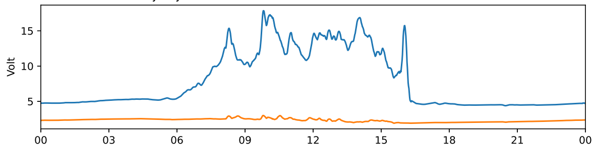
Tjautjas 30 MHz and 38 MHz riometer 2025-03-04 UTC
