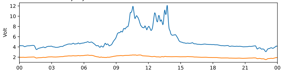
Tjautjas 30 MHz and 38 MHz riometer 2025-01-18 UTC
