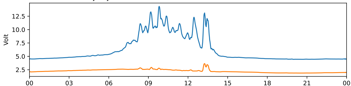
Tjautjas 30 MHz and 38 MHz riometer 2025-01-27 UTC
