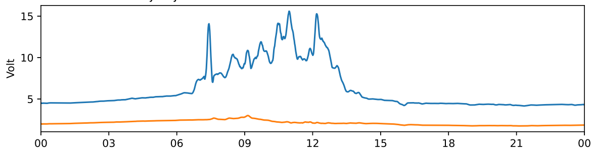
Tjautjas 30 MHz and 38 MHz riometer 2025-01-28 UTC
