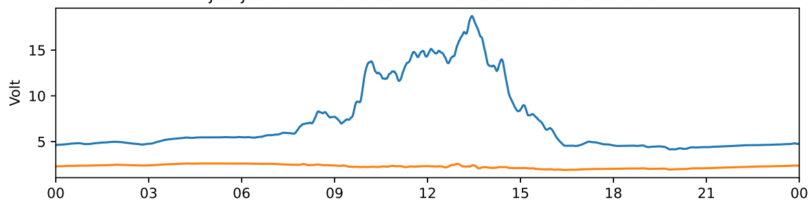
Tjautjas 30 MHz and 38 MHz riometer 2025-03-07 UTC
