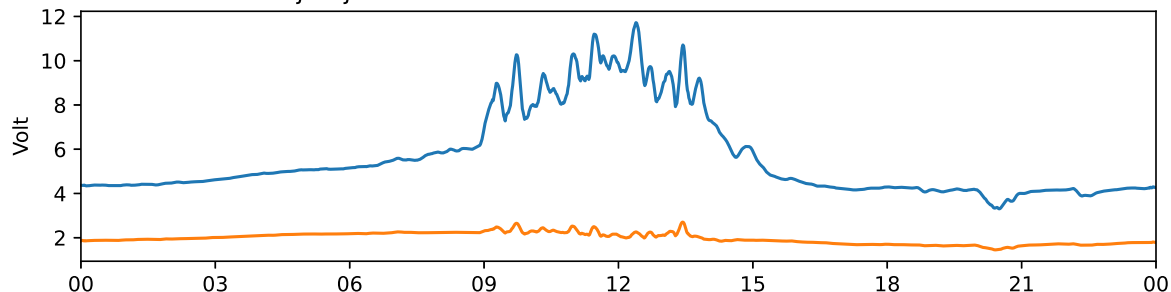
Tjautjas 30 MHz and 38 MHz riometer 2025-01-29 UTC
