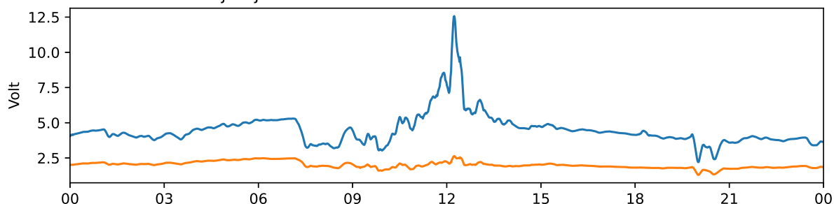
Tjautjas 30 MHz and 38 MHz riometer 2025-02-11 UTC
