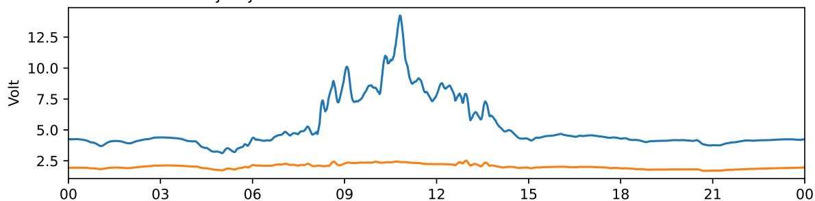
Tjautjas 30 MHz and 38 MHz riometer 2025-01-17 UTC
