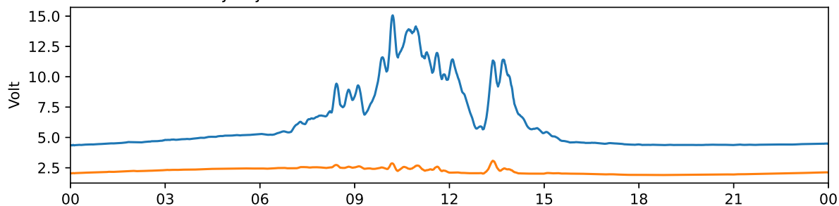
Tjautjas 30 MHz and 38 MHz riometer 2025-02-08 UTC
