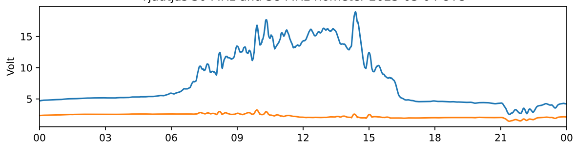
Tjautjas 30 MHz and 38 MHz riometer 2025-03-05 UTC
