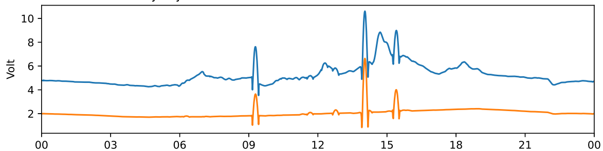
Tjautjas 30 MHz and 38 MHz riometer 2024-09-07 UTC
