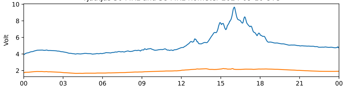
Tjautjas 30 MHz and 38 MHz riometer 2024-09-10 UTC
