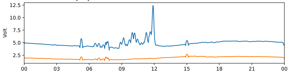
Tjautjas 30 MHz and 38 MHz riometer 2024-08-11 UTC
