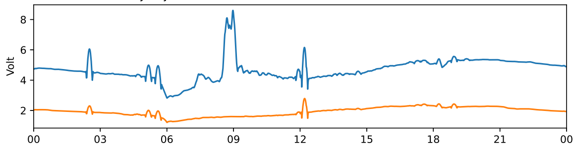
Tjautjas 30 MHz and 38 MHz riometer 2024-08-11 UTC
