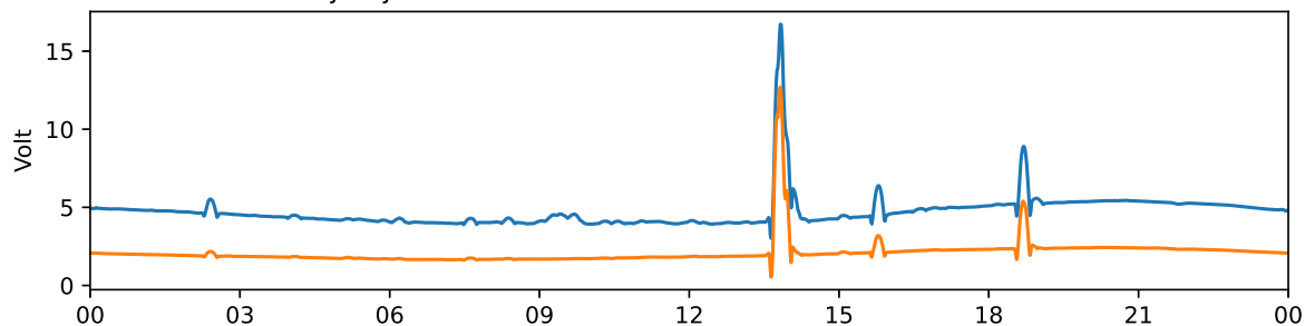
Tjautjas 30 MHz and 38 MHz riometer 2024-08-08 UTC
