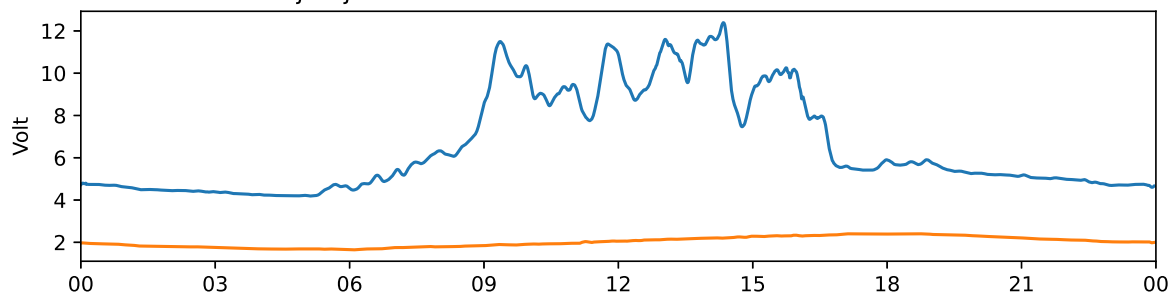
Tjautjas 30 MHz and 38 MHz riometer 2024-09-09 UTC
