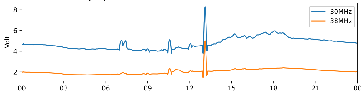
Tjautjas 30 MHz and 38 MHz riometer 2024-09-06 UTC
