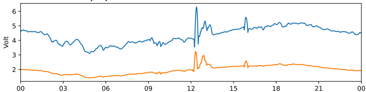
Tjautjas 30 MHz and 38 MHz riometer 2024-09-02 UTC
