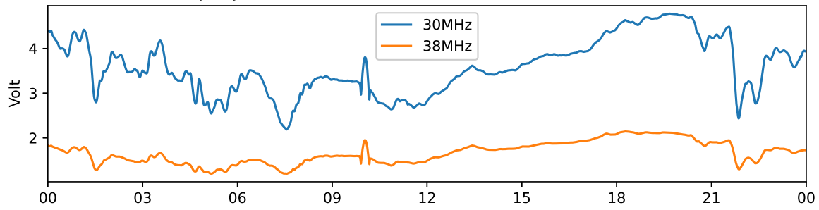
Tjautjas 30 MHz and 38 MHz riometer 2024-09-18 UTC
