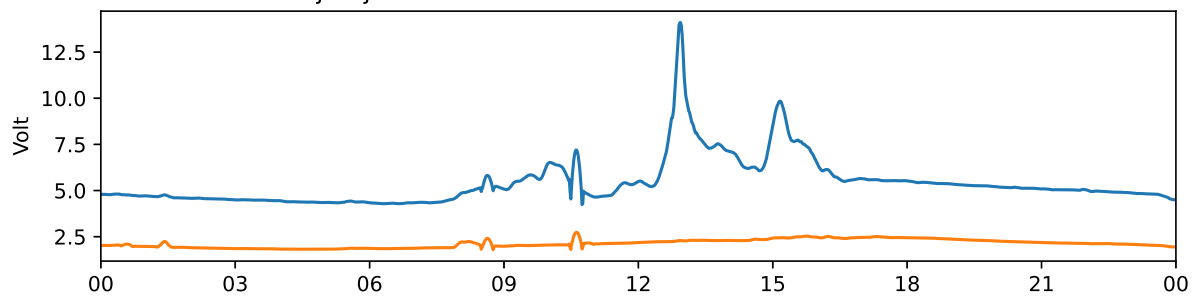
Tjautjas 30 MHz and 38 MHz riometer 2024-09-22 UTC
