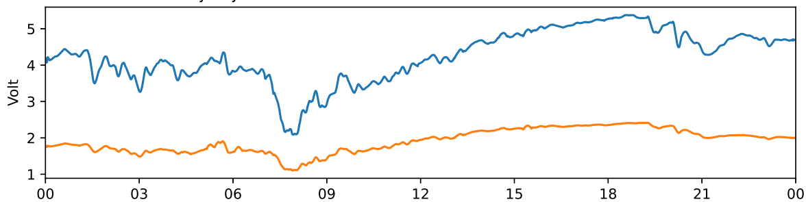
Tjautjas 30 MHz and 38 MHz riometer 2024-09-01 UTC
