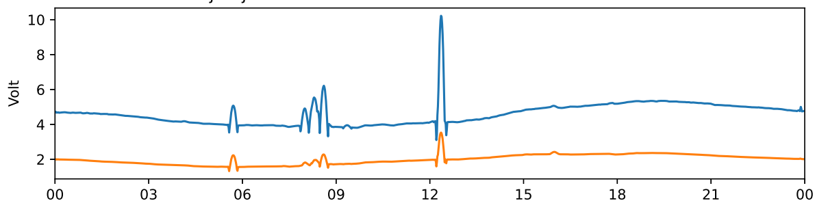
Tjautjas 30 MHz and 38 MHz riometer 2024-09-04 UTC
