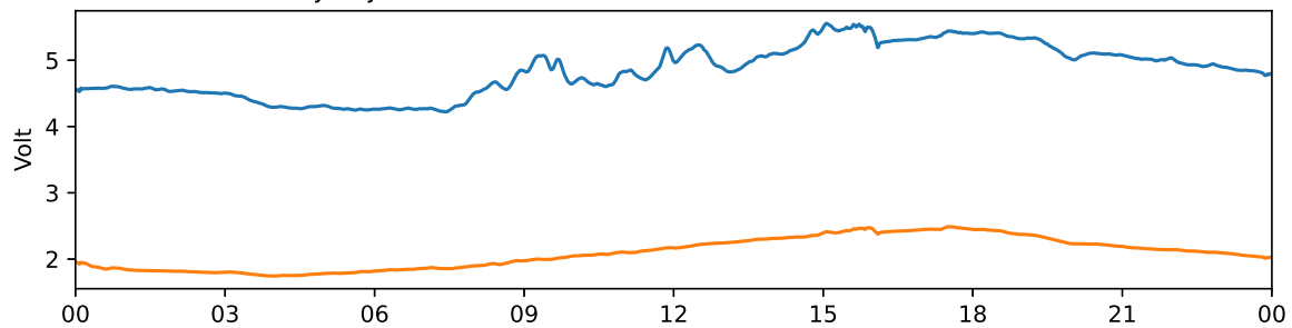
Tjautjas 30 MHz and 38 MHz riometer 2024-09-22 UTC
