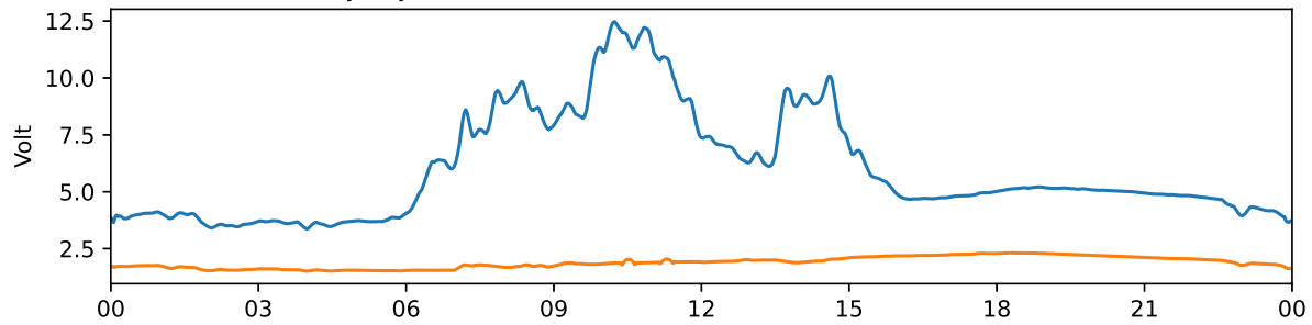
Tjautjas 30 MHz and 38 MHz riometer 2024-09-19 UTC
