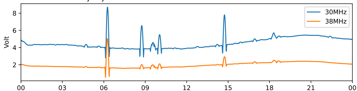
Tjautjas 30 MHz and 38 MHz riometer 2024-08-07 UTC
