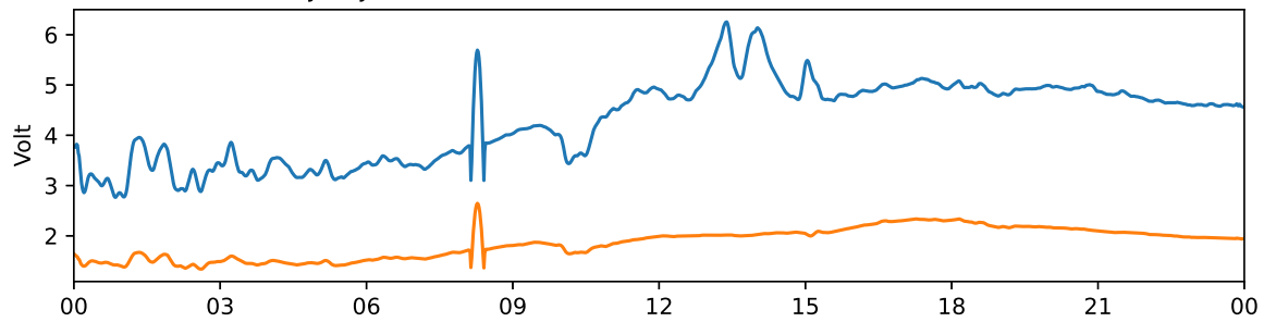
Tjautjas 30 MHz and 38 MHz riometer 2024-09-20 UTC
