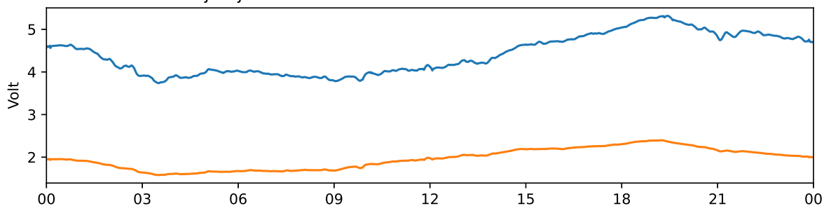
Tjautjas 30 MHz and 38 MHz riometer 2024-09-03 UTC
