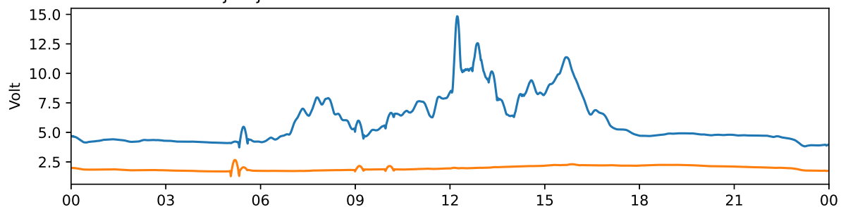
Tjautjas 30 MHz and 38 MHz riometer 2024-09-10 UTC
