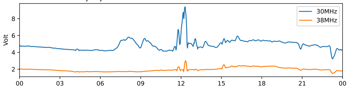
Tjautjas 30 MHz and 38 MHz riometer 2024-08-31 UTC
