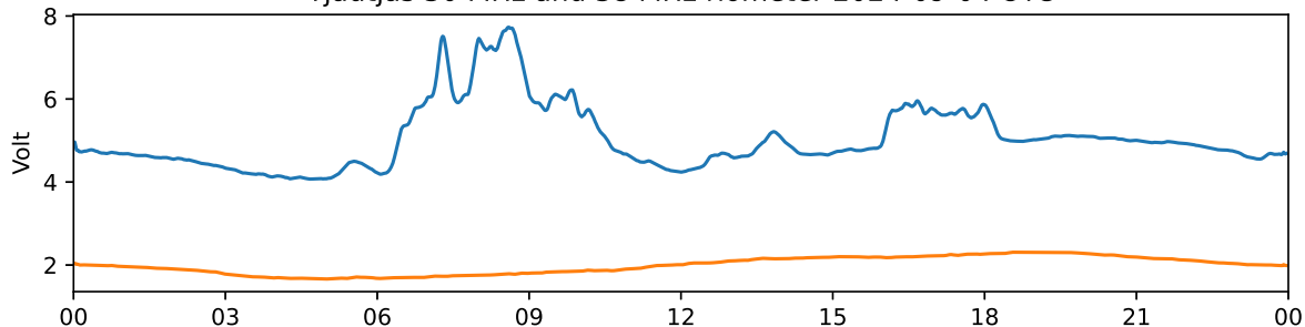
Tjautjas 30 MHz and 38 MHz riometer 2024-09-04 UTC
