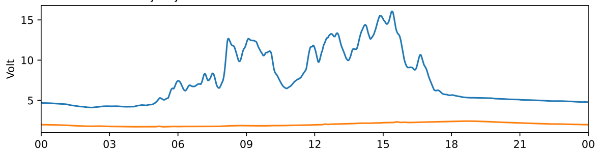
Tjautjas 30 MHz and 38 MHz riometer 2024-09-08 UTC
