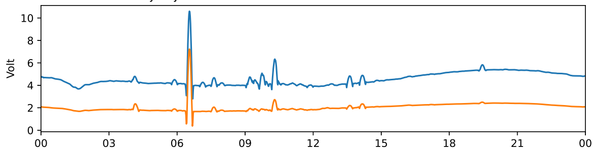
Tjautjas 30 MHz and 38 MHz riometer 2024-08-09 UTC
