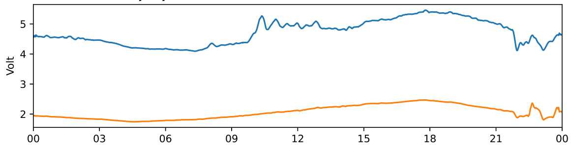
Tjautjas 30 MHz and 38 MHz riometer 2024-09-21 UTC
