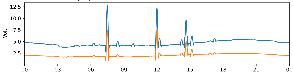
Tjautjas 30 MHz and 38 MHz riometer 2024-08-10 UTC
