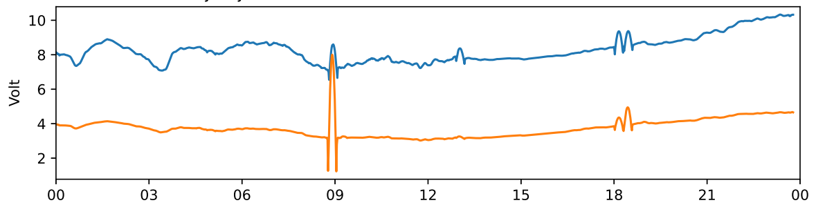
Tjautjas 30 MHz and 38 MHz riometer 2023-05-12 UTC
