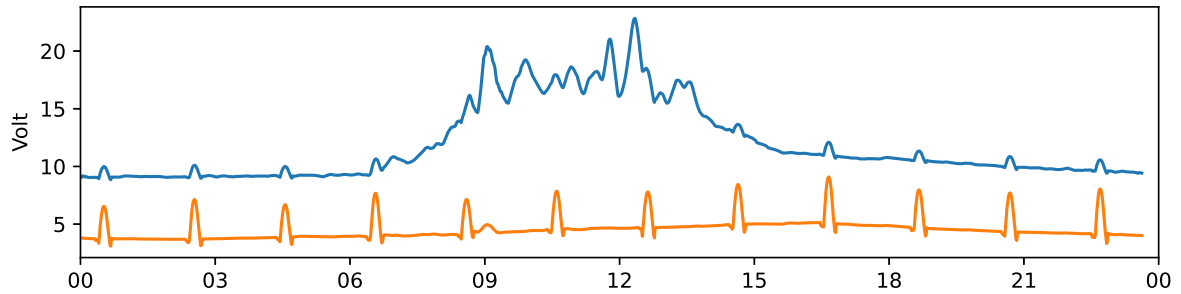
Tjautjas 30 MHz and 38 MHz riometer 2022-10-18 UTC
