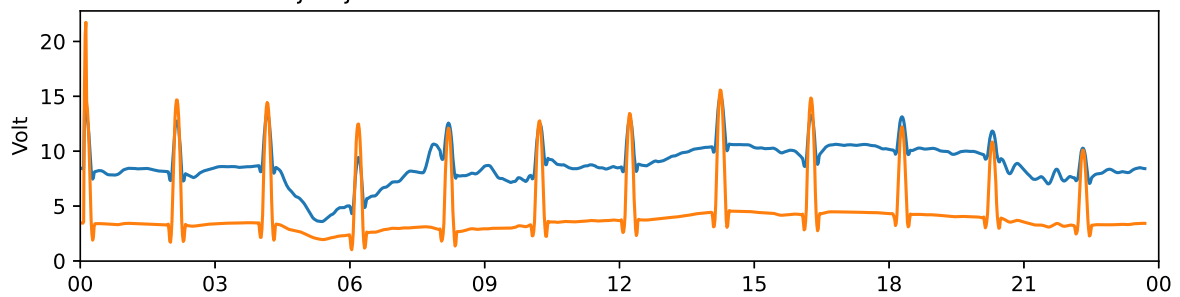
Tjautjas 30 MHz and 38 MHz riometer 2022-10-06 UTC
