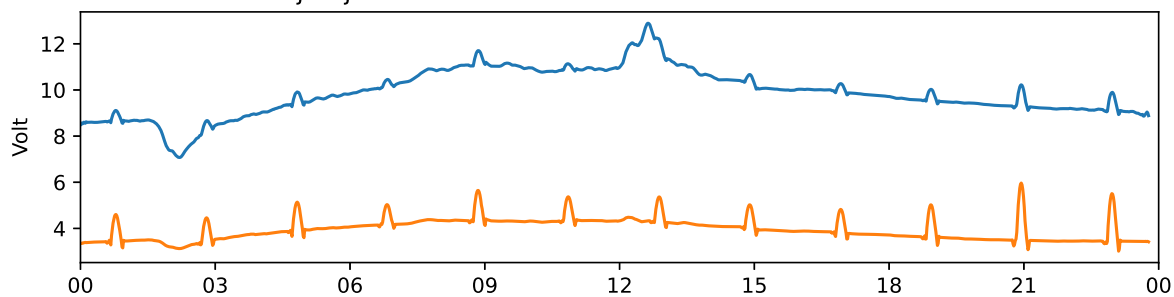
Tjautjas 30 MHz and 38 MHz riometer 2022-12-29 UTC
