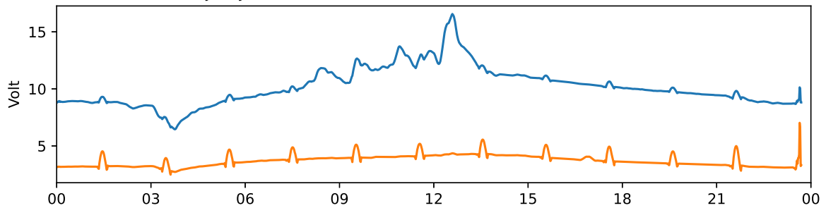
Tjautjas 30 MHz and 38 MHz riometer 2022-11-22 UTC
