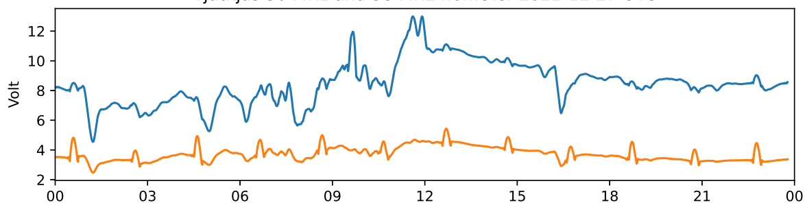
Tjautjas 30 MHz and 38 MHz riometer 2022-12-28 UTC
