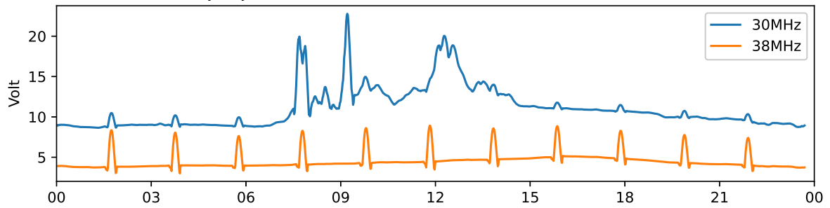
Tjautjas 30 MHz and 38 MHz riometer 2022-10-14 UTC
