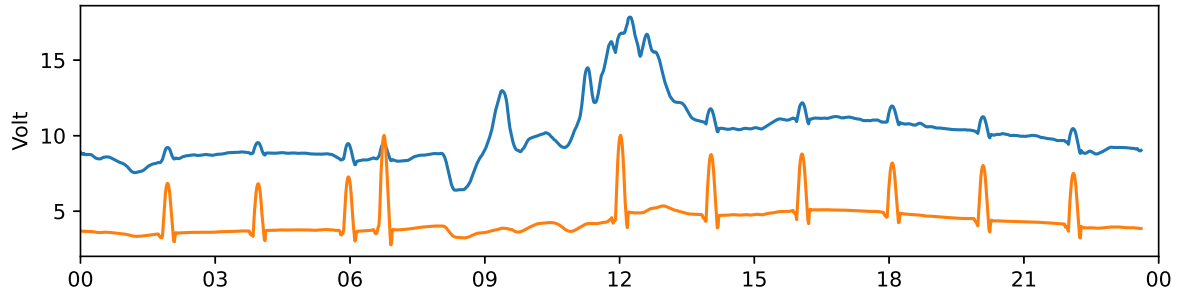
Tjautjas 30 MHz and 38 MHz riometer 2022-10-15 UTC
