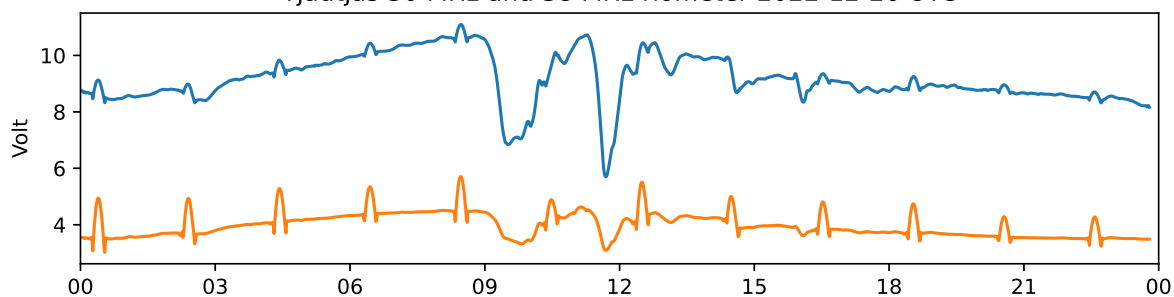
Tjautjas 30 MHz and 38 MHz riometer 2022-12-27 UTC
