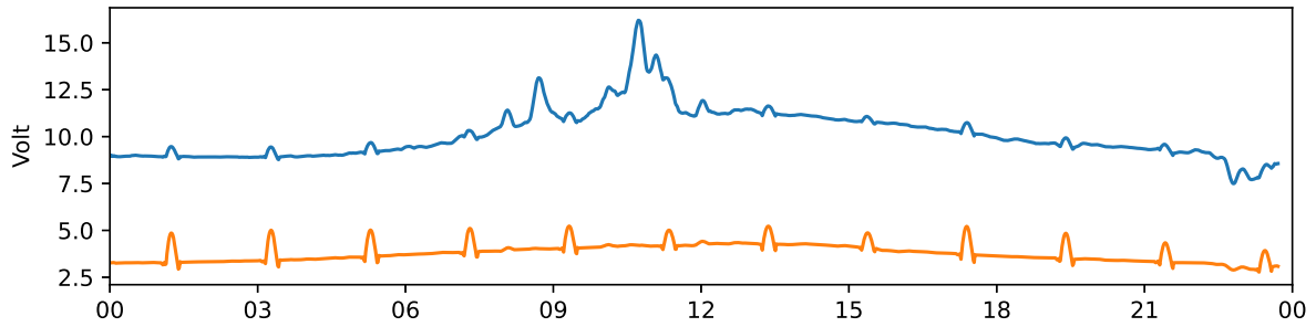
Tjautjas 30 MHz and 38 MHz riometer 2022-11-21 UTC
