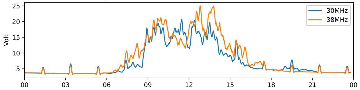
Tjautjas 30 MHz and 38 MHz riometer 2022-10-02 UTC
