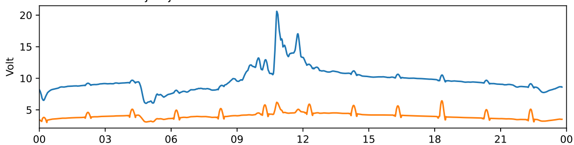
Tjautjas 30 MHz and 38 MHz riometer 2022-12-26 UTC
