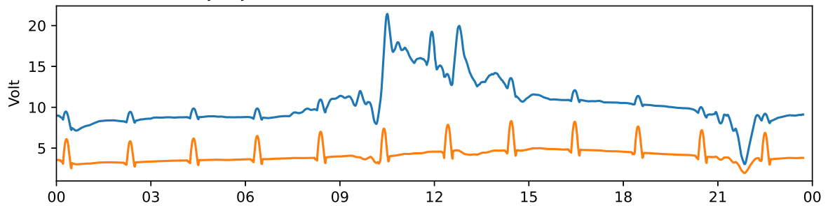
Tjautjas 30 MHz and 38 MHz riometer 2022-10-17 UTC
