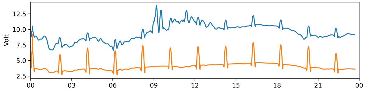
Tjautjas 30 MHz and 38 MHz riometer 2022-10-16 UTC
