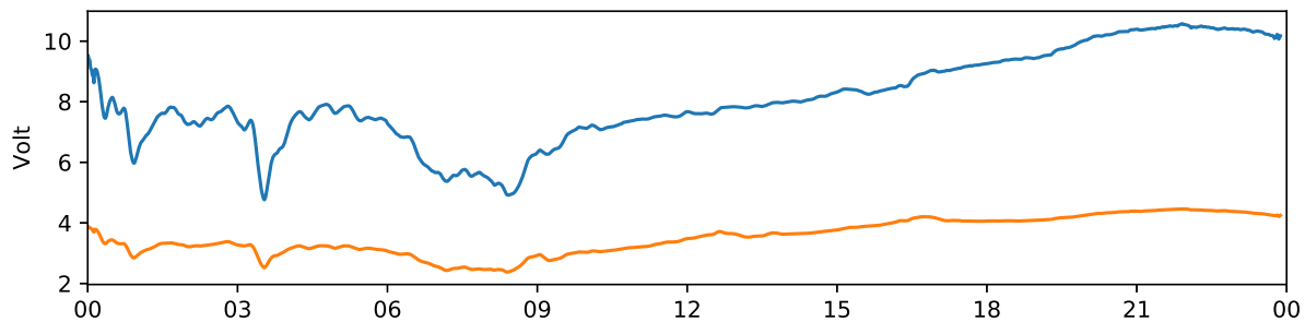
Kiruna 30 MHz and 38 MHz riometer 2020-07-15 UTC
