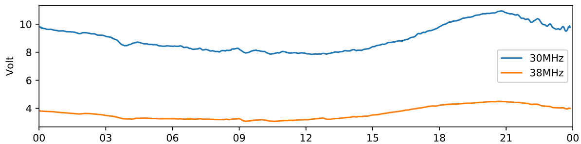
Kiruna 30 MHz and 38 MHz riometer 2020-07-14 UTC
