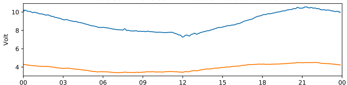
Kiruna 30 MHz and 38 MHz riometer 2020-07-17 UTC
