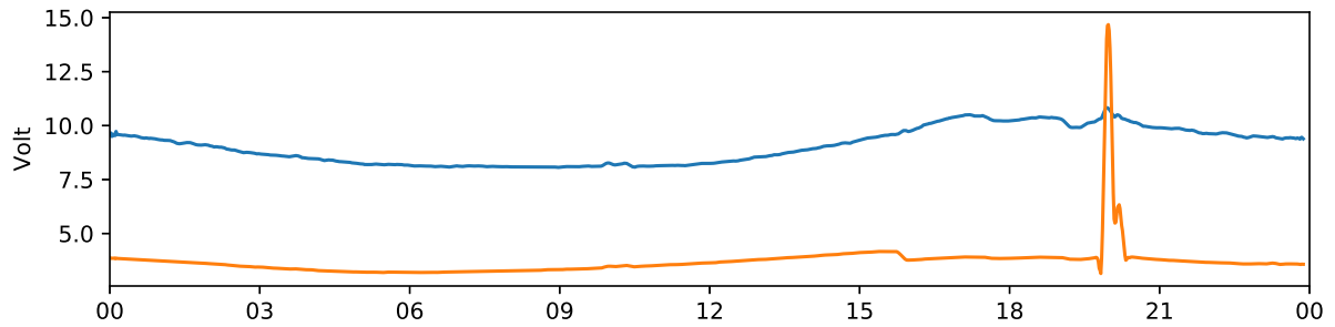
Kiruna 30 MHz and 38 MHz riometer 2020-08-22 UTC
