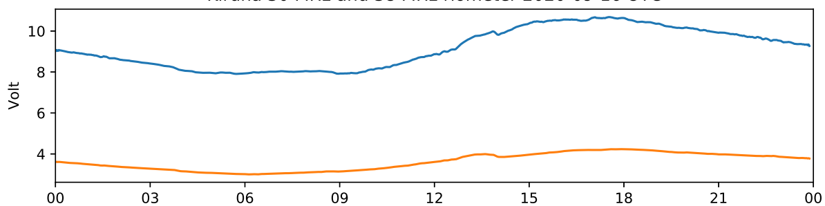
Kiruna 30 MHz and 38 MHz riometer 2020-09-16 UTC
