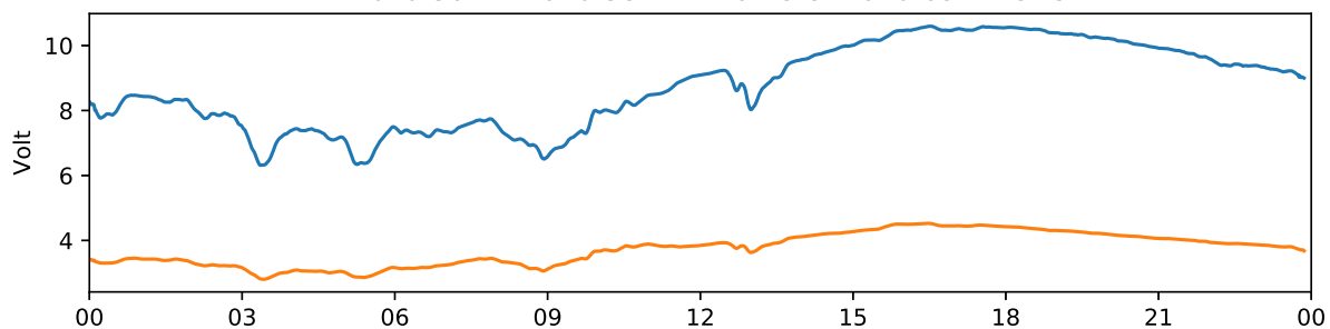
Kiruna 30 MHz and 38 MHz riometer 2020-09-15 UTC
