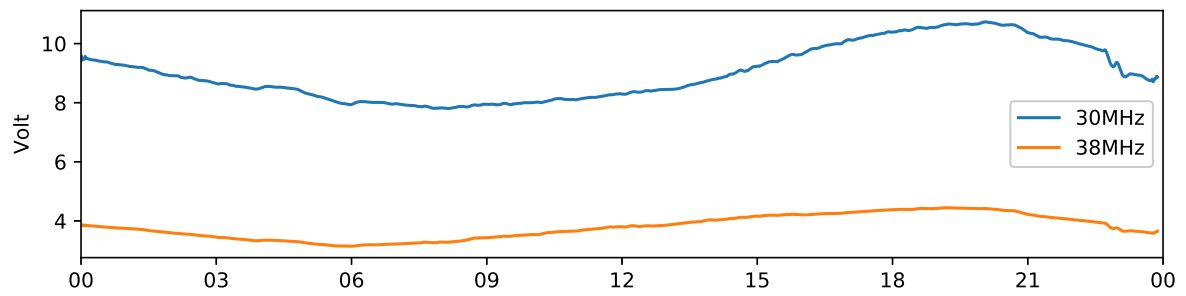
Kiruna 30 MHz and 38 MHz riometer 2020-08-19 UTC
