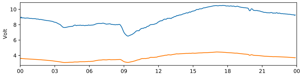
Kiruna 30 MHz and 38 MHz riometer 2020-09-13 UTC
