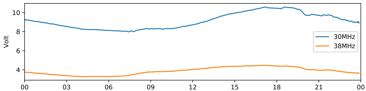
Kiruna 30 MHz and 38 MHz riometer 2020-09-12 UTC
