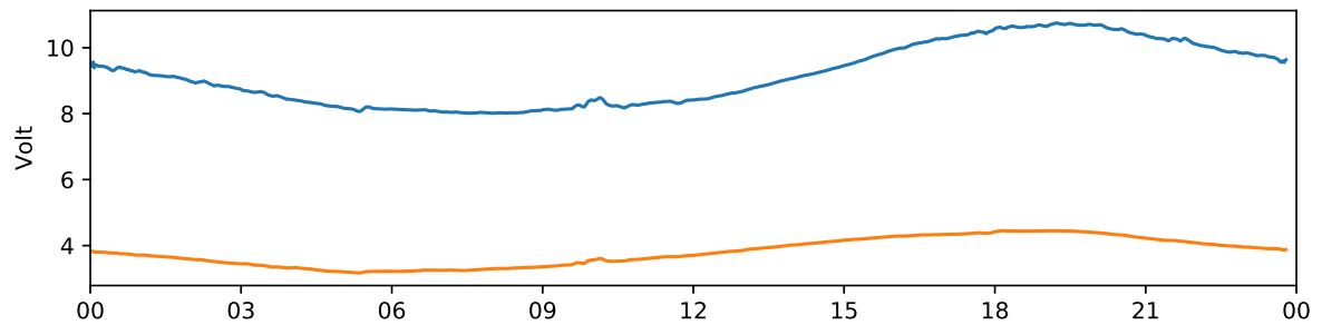
Kiruna 30 MHz and 38 MHz riometer 2020-08-21 UTC
