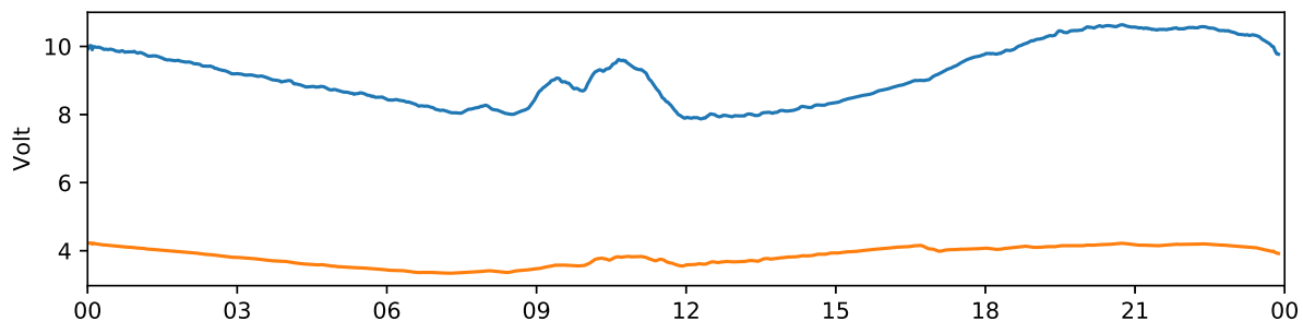
Kiruna 30 MHz and 38 MHz riometer 2020-07-18 UTC
