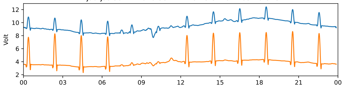
Tjautjas 30 MHz and 38 MHz riometer 2022-09-16 UTC
