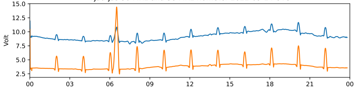
Tjautjas 30 MHz and 38 MHz riometer 2022-09-15 UTC
