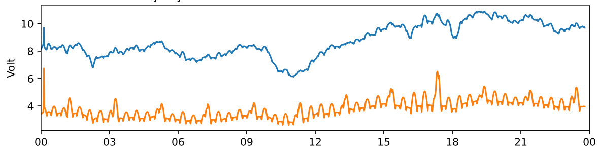
Tjautjas 30 MHz and 38 MHz riometer 2022-08-22 UTC
