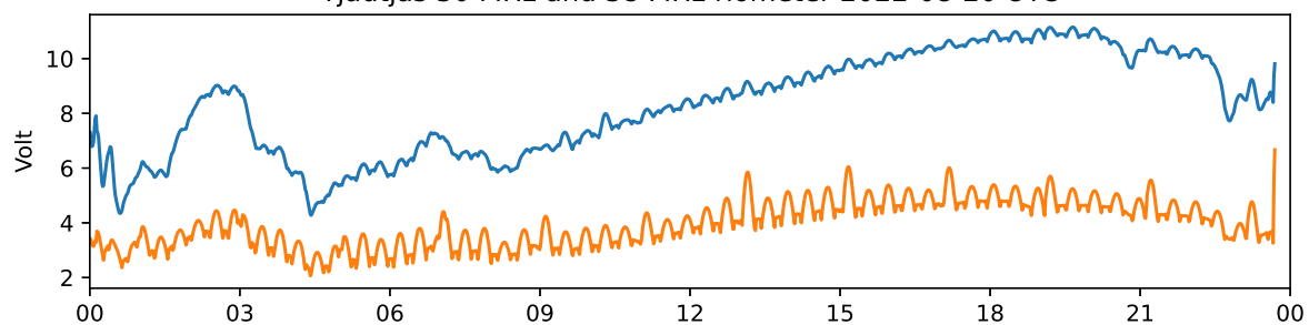
Tjautjas 30 MHz and 38 MHz riometer 2022-08-21 UTC
