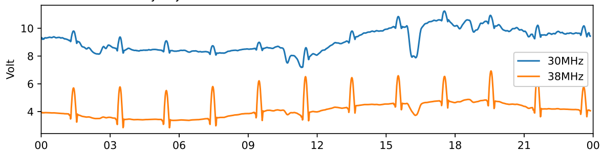
Tjautjas 30 MHz and 38 MHz riometer 2022-09-12 UTC
