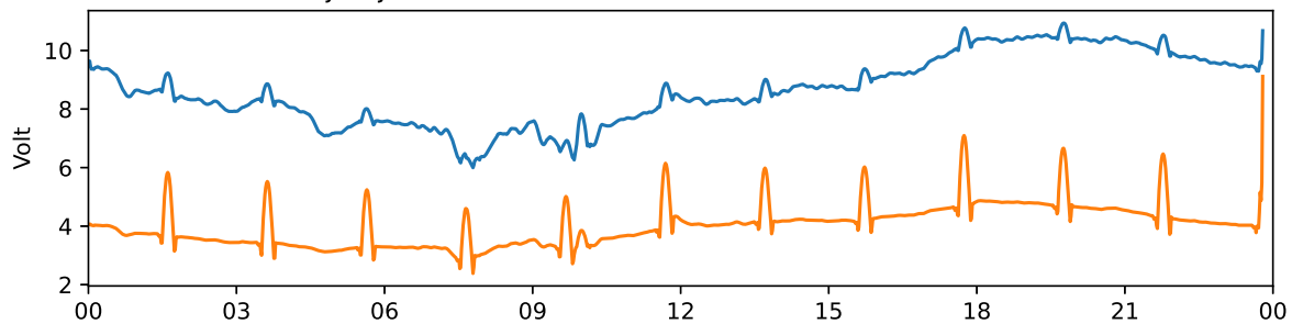
Tjautjas 30 MHz and 38 MHz riometer 2022-09-13 UTC
