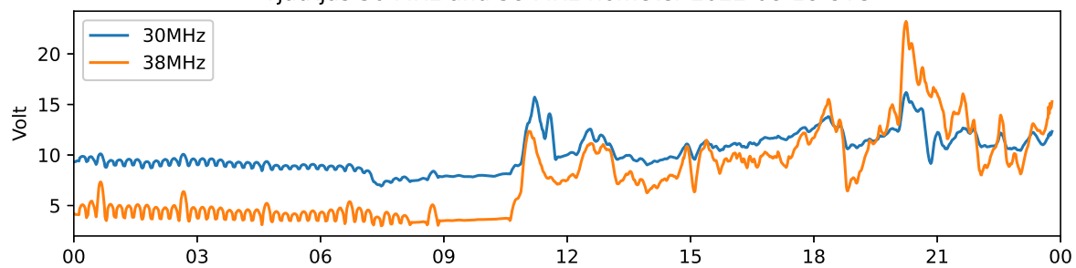
Tjautjas 30 MHz and 38 MHz riometer 2022-08-19 UTC
