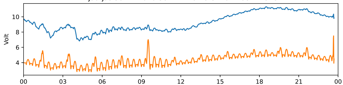
Tjautjas 30 MHz and 38 MHz riometer 2022-08-23 UTC
