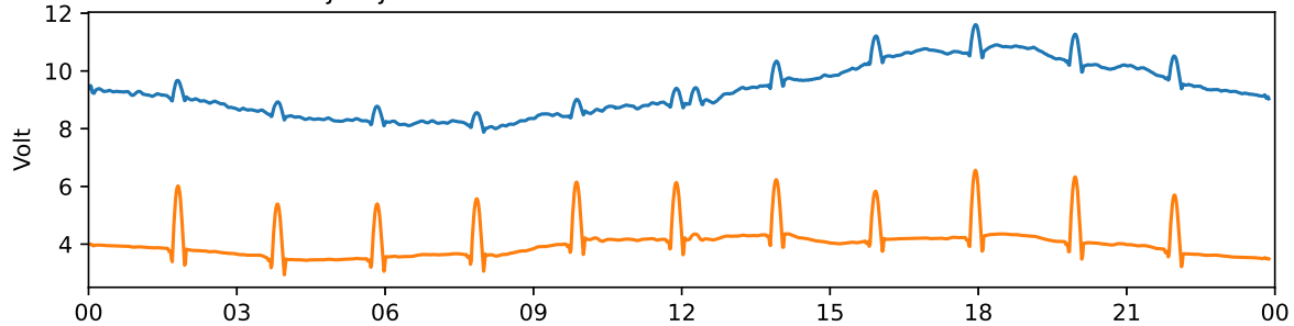
Tjautjas 30 MHz and 38 MHz riometer 2022-09-14 UTC
