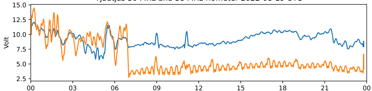
Tjautjas 30 MHz and 38 MHz riometer 2022-08-20 UTC
