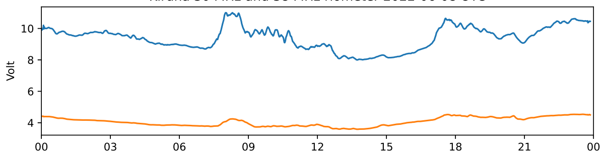
Kiruna 30 MHz and 38 MHz riometer 2022-06-08 UTC
