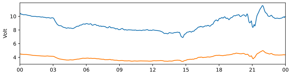
Kiruna 30 MHz and 38 MHz riometer 2022-06-07 UTC
