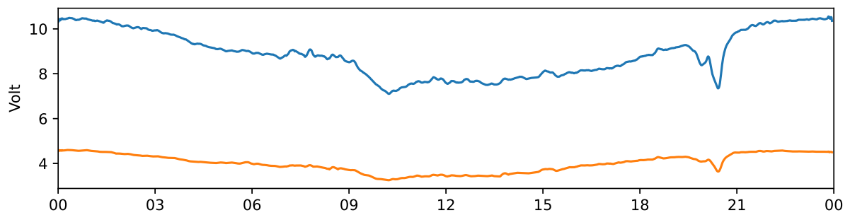
Kiruna 30 MHz and 38 MHz riometer 2022-06-06 UTC
