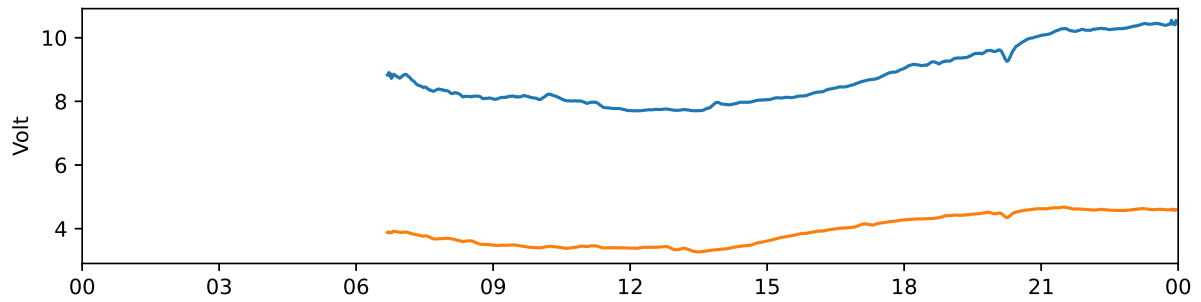
Kiruna 30 MHz and 38 MHz riometer 2022-06-05 UTC
