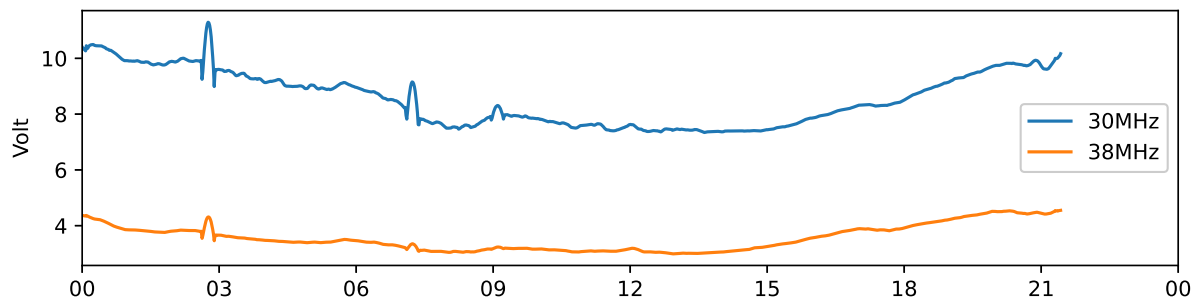
Kiruna 30 MHz and 38 MHz riometer 2022-06-04 UTC
