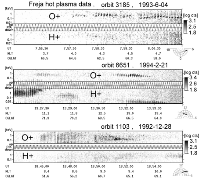
Figure 3. Energy-time spectrograms for heavy ions and protons observed by Freja at about 1700 km altitude [after Yamauchi et al., 2005a].
