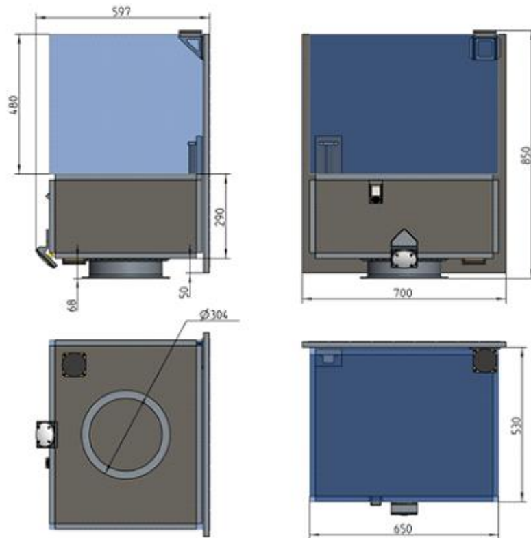
Figure 4-2: InnoSat basic dimensions
