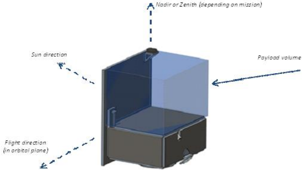
Figure 4-1: Satellite baseline configuration and available payload volume
